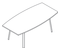
PLF12P 2000 / 800-1000 / 740 46.5 kg
