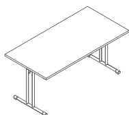
PSU07 1390 / 695 / 725 23 kg
